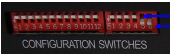
Figure 2 Auxiliary DIP switches
